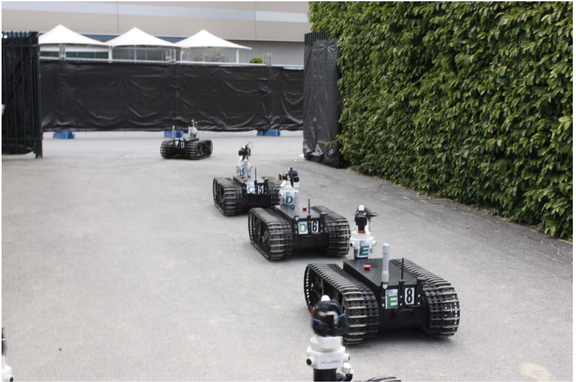
The first of the RASR team of robots crosses the line to start Phase One of the MAGIC Grand Challenge.
